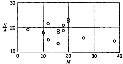
FIG. 10-31.— N/A as a function of N .
